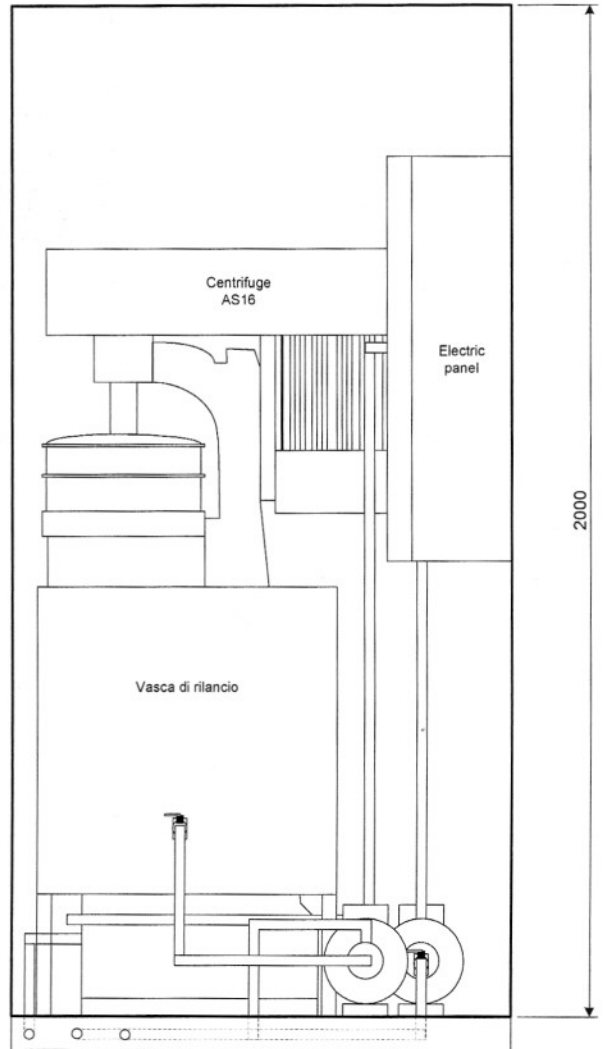
End view
