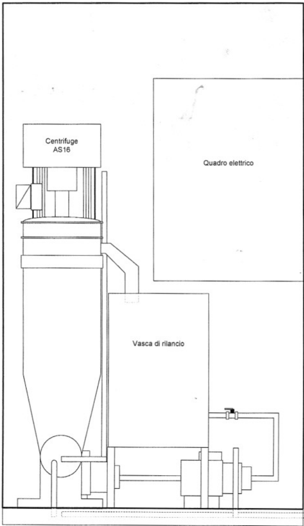
Elevation View
